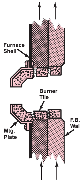
Figure 3. Tile shears off due to unequal expansion of refractory and shell or unequal expansion between layers of refractory brickwork and matrix around tile prevent this.
