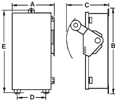
2723 Fusible Disconnect Switch*
